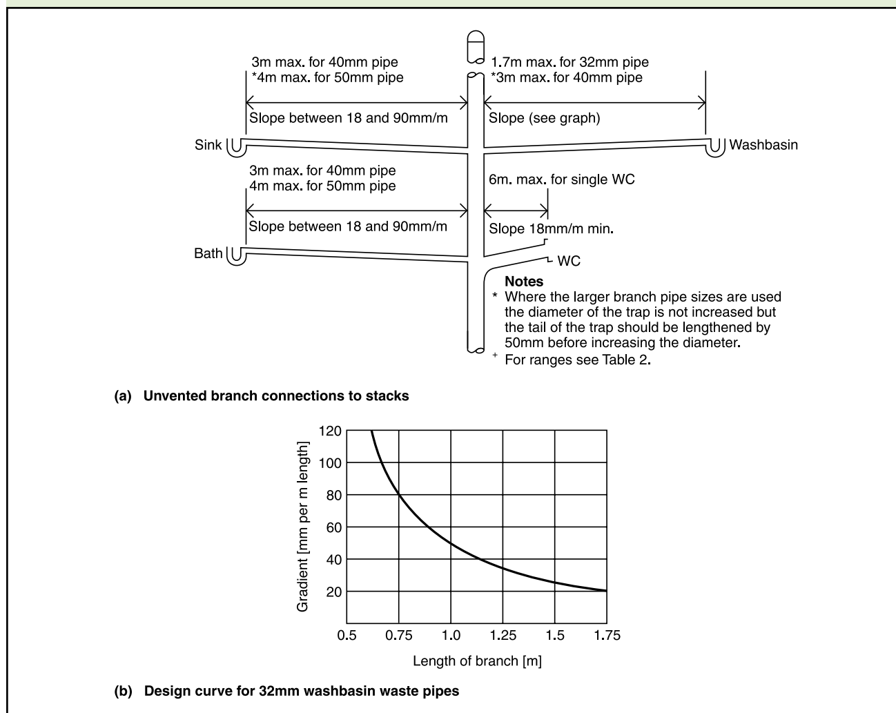
Diagram 3 Branch connections
