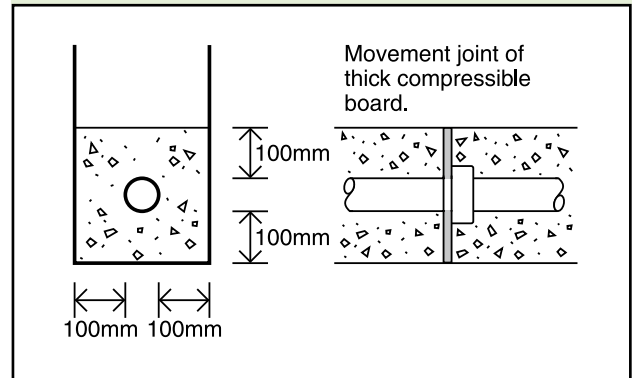
Diagram 12 Joints for concrete encased pipes (minimum sizes)
